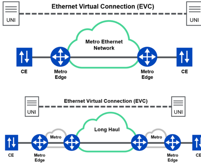
Figure 1: General Metro Architecture and Components.
